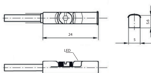
Dimensions [mm]
